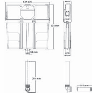
concealed cistern Code 62 L 547 W 90 H 574mm / L 21.5" W 3.5" H 22.5"
